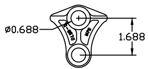
BASE VIEW
