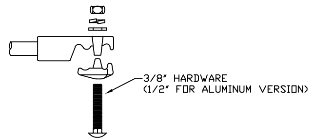
END FITTING VIEW (TOP VIEW)
