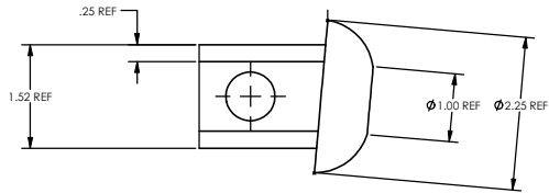
DETAIL A
