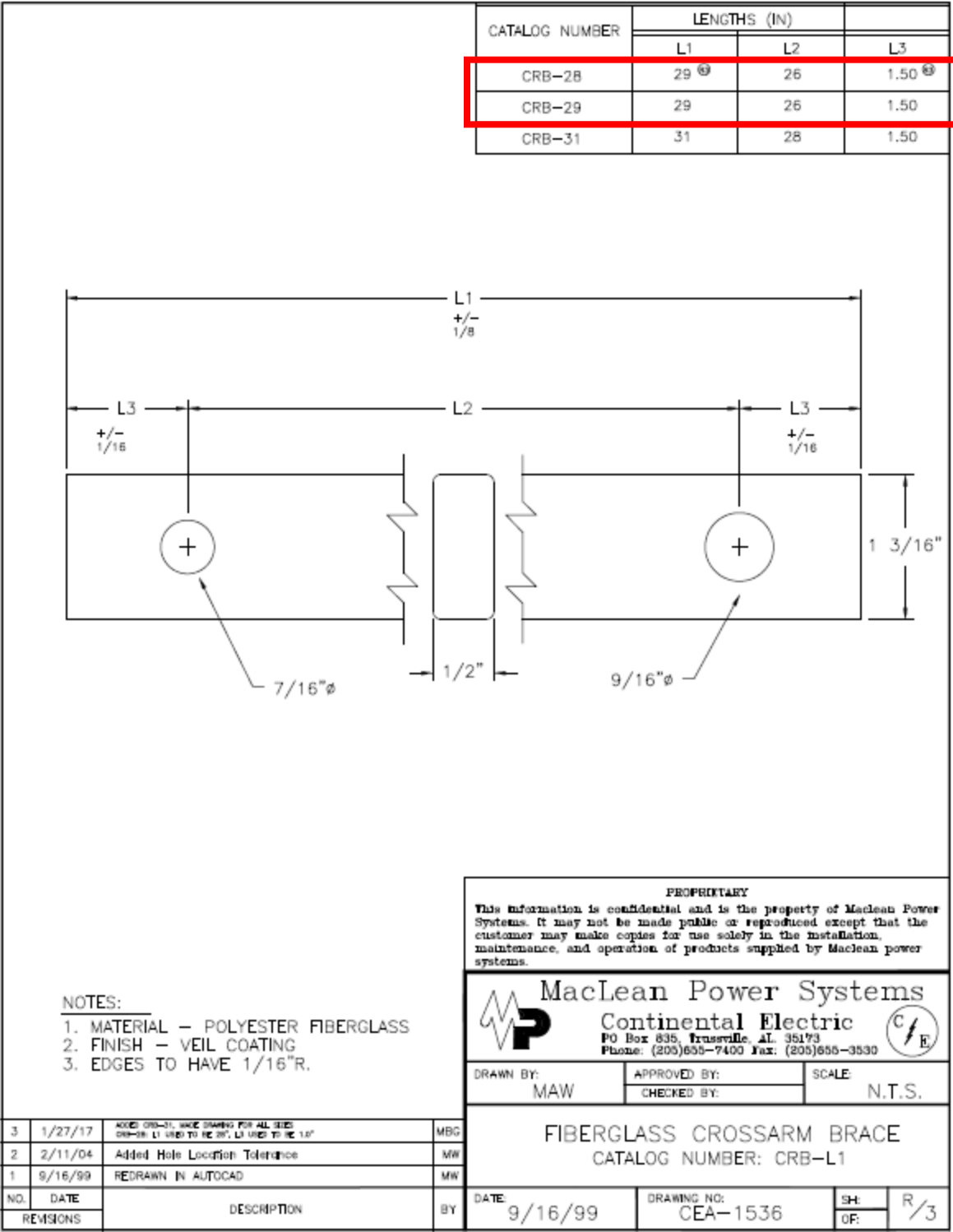
Figure 1 – Drawing of CRB28 and CRB29
