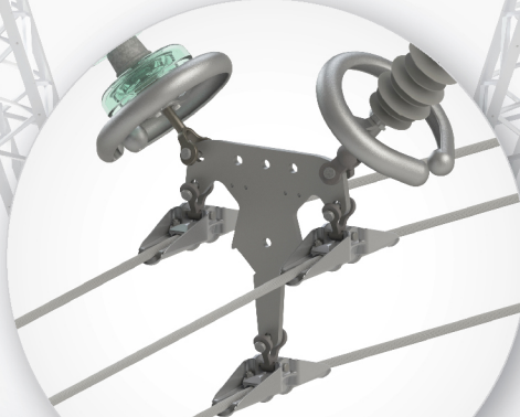
3 Conductor Bundle, V-String with Formula Clamps
