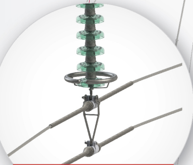
Vertical Bundle w/ Helical Suspension Clamps
